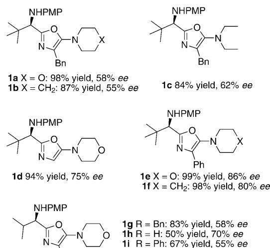
Figure 1. General reaction conditions: preformed imine 6 / 4 = 1:1 ( 6 not shown), in toluene c = 0.05 M, 5 (0.2 equiv). Yield refers to chromatographically pure material; ee value was determined by chiral HPLC analysis. Catalyst 5l was used for the preparation of 1a–1c and catalyst 5g was used for the preparation of 1d–1i .
